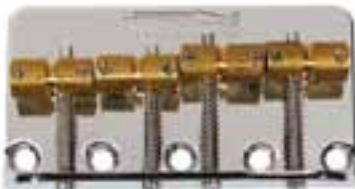
Wilkinson bridge-tailpiece JB-Pucher bass, pitch 19mm, brass saddles
